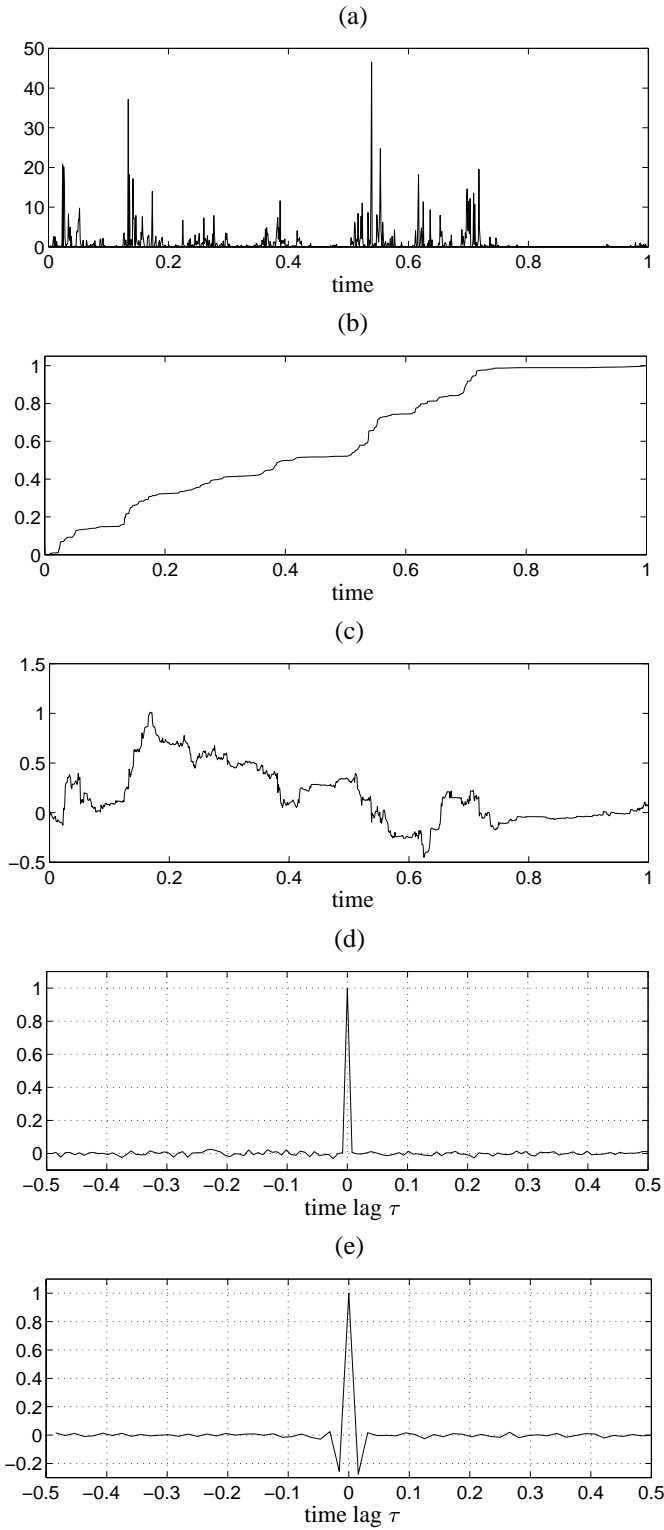
FIG. 1: (a) Increments of one realization of a Binomial cascade \mathcal{M}((k+1)2^j) - \mathcal{M}(k2^j) = \mu([k2^j, (k+1)2^j]) , ( k = 0, \dots, 2^j - 1 ). (b) Realization of a Binomial cascade \mathcal{M}(k2^j) , ( k = 0, \dots, 2^j - 1 ). (c) One realization of ordinary Brownian motion warped with the realization of (b), i.e. \mathcal{B}(k2^j) = B_{1/2}(\mathcal{M}(k2^j)) ( k = 0, \dots, 2^j - 1 ). (d) Empirical residual correlation of the wavelet decomposition of \mathcal{B}(t) using a Haar wavelet. (e) Empirical residual correlation of the wavelet decomposition of \mathcal{B}(t) using a Daubechies wavelet with regularity 2.
